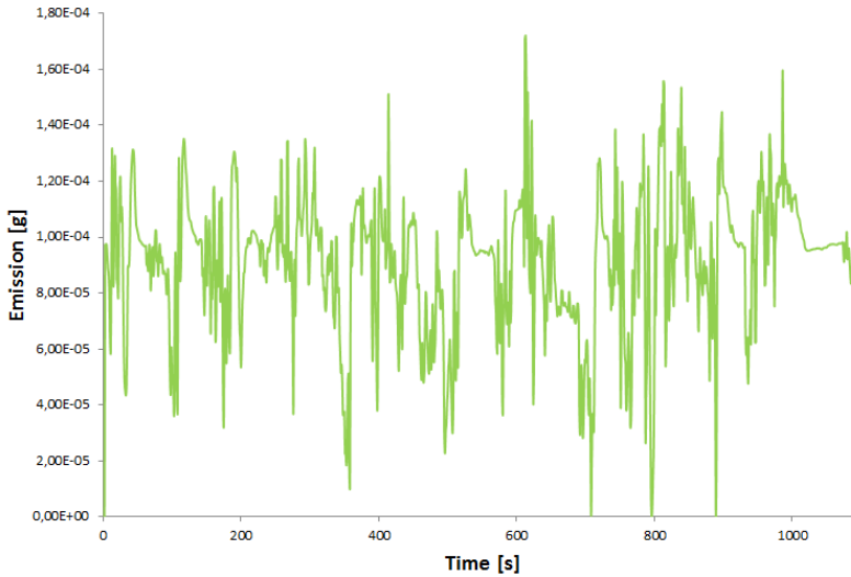
Fig. 11. Particulate matter emission per second obtained during economic drive
