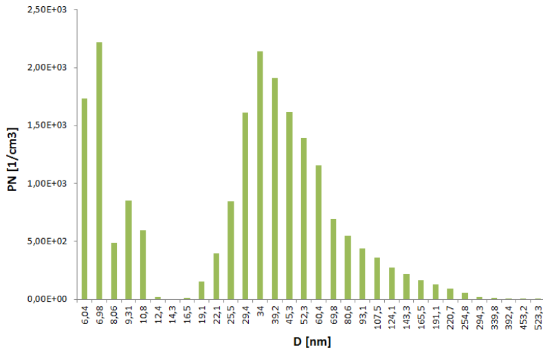
Fig. 9. Dimensional distribution of PN during economic drive
