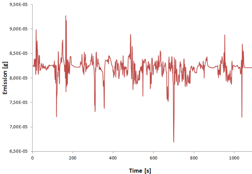
Fig. 10. Particulate matter emission per second obtained during dynamic drive
