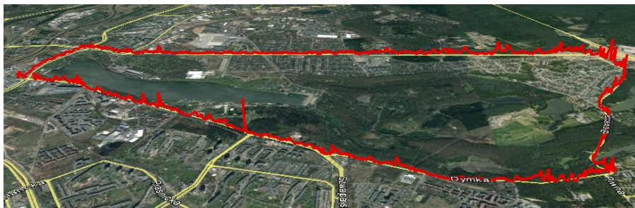
Fig. 5. Total concentration of PM during economic drive
