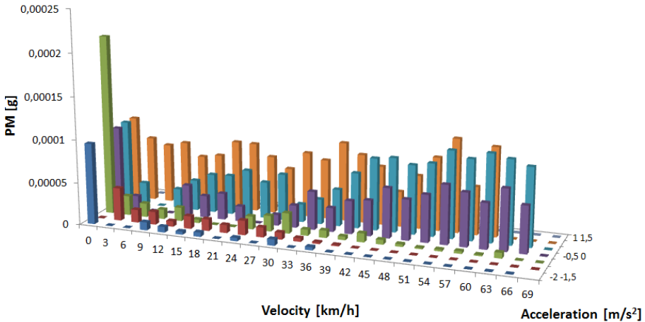
Fig. 12. Emission of PM in the range of vehicle speed and acceleration during dynamic drive
