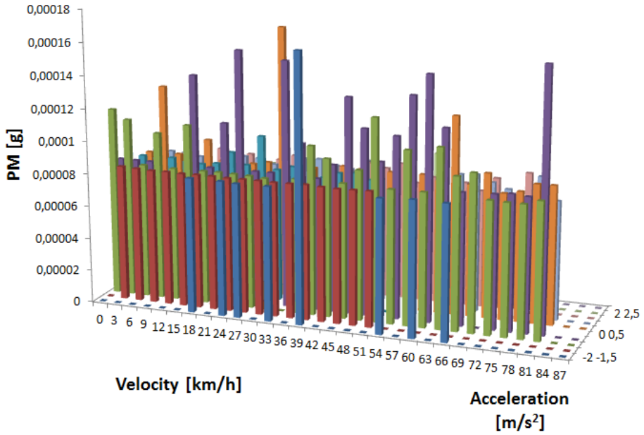
Fig. 13. Emission of PM in the range of vehicle speed and acceleration during economic drive
