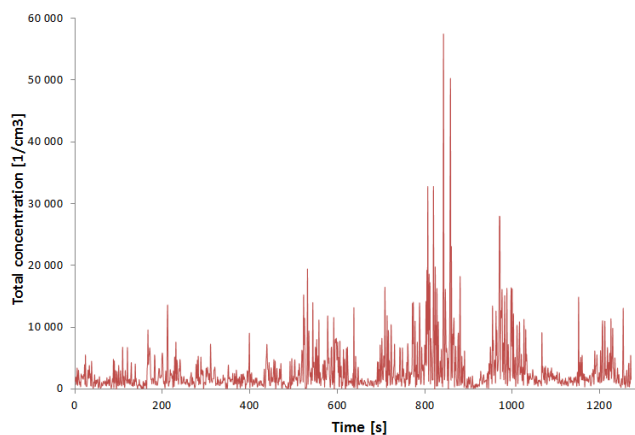
Fig. 6. Total concentration of PM during dynamic drive
