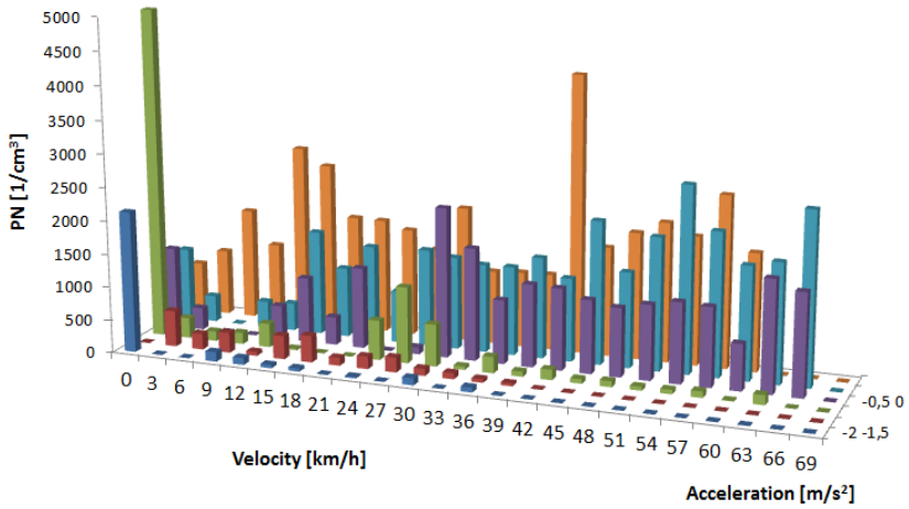
Fig. 14. Emission of PN in the range of vehicle speed and acceleration during economic drive
