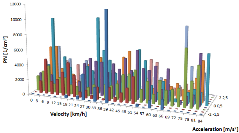
Fig. 15. Emission of PN in the range of vehicle speed and acceleration during economic drive Average results of tests with comparison to norms were shown in Table 3.
