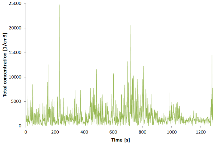
Fig. 7. Total concentration of PM during economic drive
