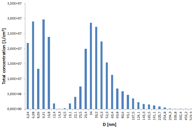
Fig. 8. Dimensional distribution of PN during dynamic drive
