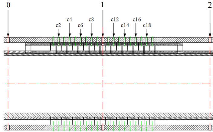
Fig. 14. Diagram of the location of the measurement planes: 0, 1, 2 and the points of measurement of static pressure in the chambers of single-sided and double-sided seals
