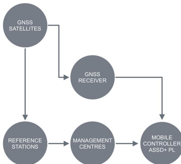
Fig. 4. Concept of information flow in the ASG-EUPOS system including the Mobile Controller ASSD+PL
