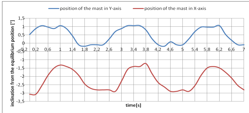
Graph 2. Position of the mast of the inverted pendulum during the stationary test [Judt 2015]
