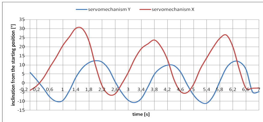
Graph 3. Position of the servomechanisms in the dynamic test [Judt 2015]
