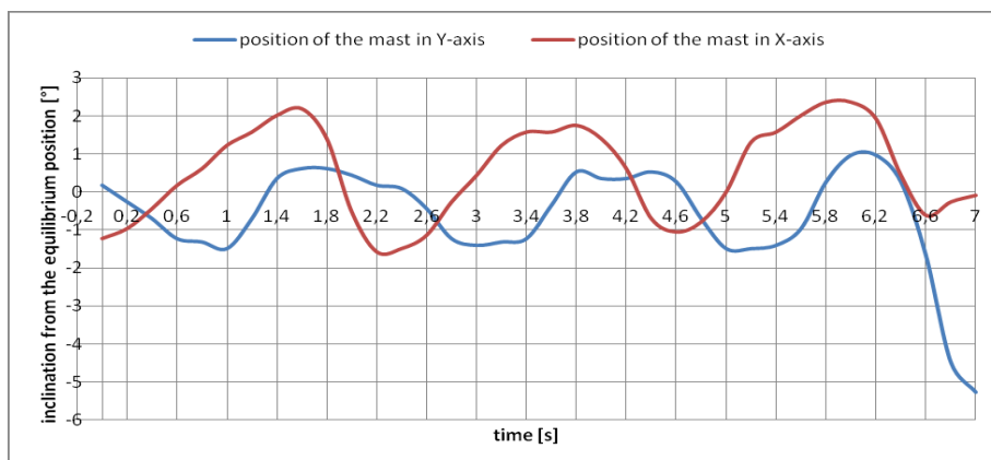
Graph 4. Position of the mast of the inverted pendulum during the dynamic test [Judt 2015]
