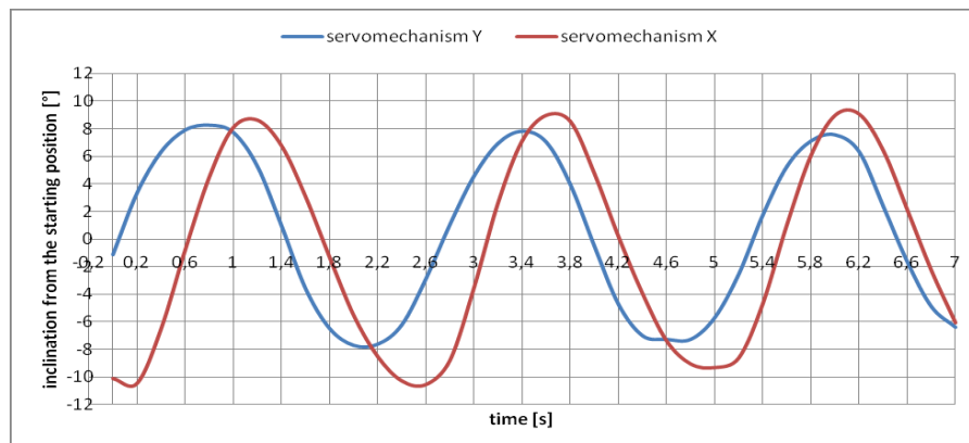
Graph 1. Position of the servomechanisms in the stationary test [Judt 2015]
